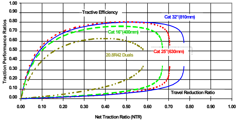
Figure 33. Belt width comparison on subsoiled land (belted tractor total weight = 12700 kg; wheel tractor axle weight = 8303 kg).
