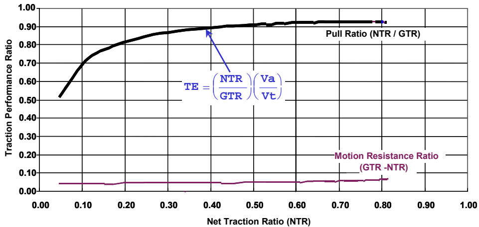
Figure 12. Pull losses in traction.
