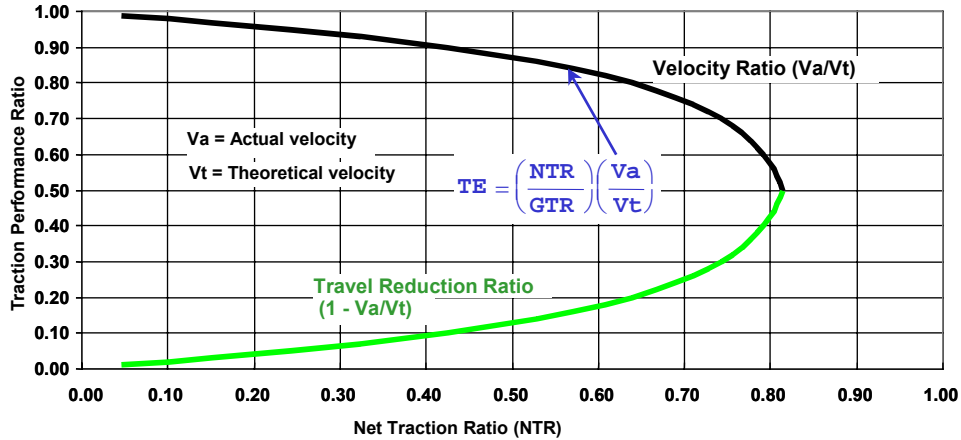
Figure 11. Velocity losses in traction.
