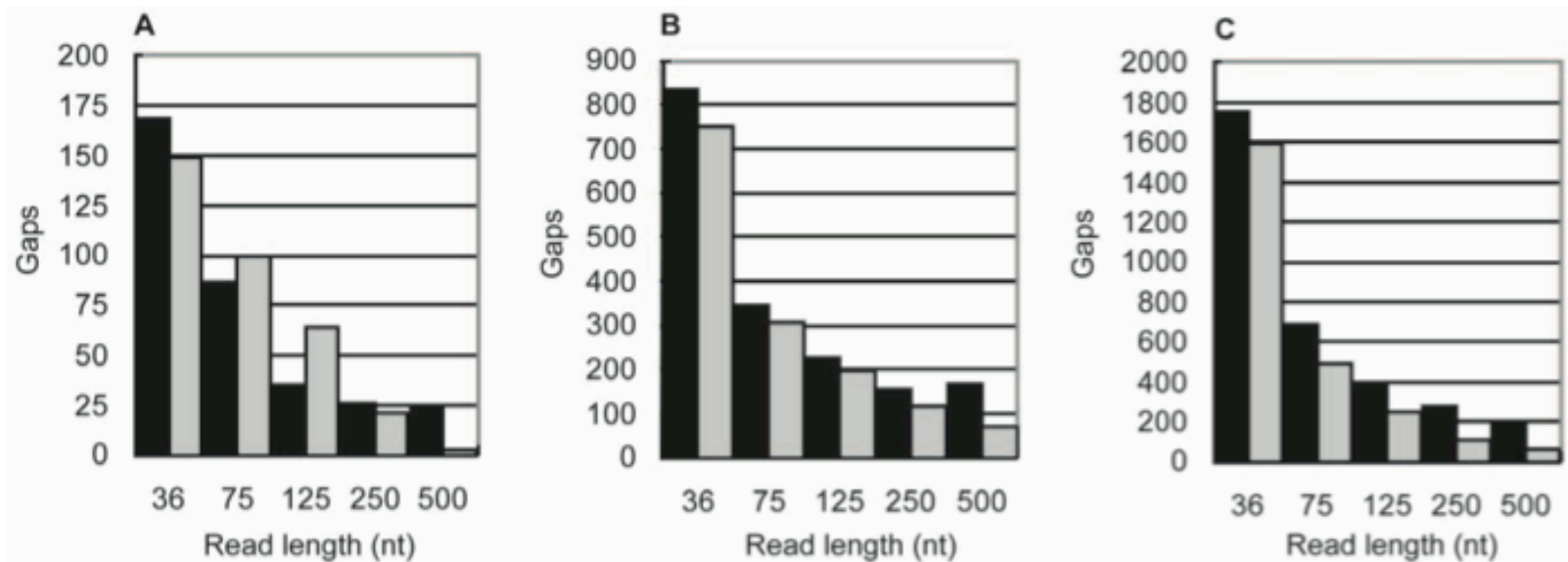
Figure 3. Assessing the accuracy of the algorithm. The number of repeat-induced gaps predicted by the algorithm (grey bars) compared to the number of gaps observed (black bars) in actual assemblies of 36, 75, 125, 250, and 500nt simulated reads from A) M. genitalium , B) E. coli and C) S. coelicolor . The observed gaps are those unique, non-redundant contigs larger than the read length. The coverage depth of each read set was the threshold at which random gaps are no longer predicted by the Lander-Waterman model. This occurs at effective coverage depths of 9–17x. doi:10.1371/journal.pone.0011518.g003
