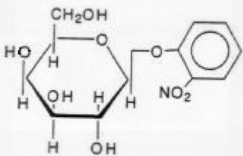
ONPG (colorless)
