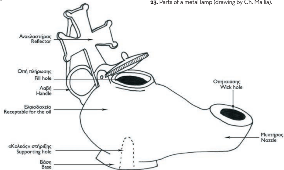
23. Parts of a metal lamp (drawing by Ch. Mallia).
