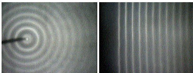
Spherical waves
