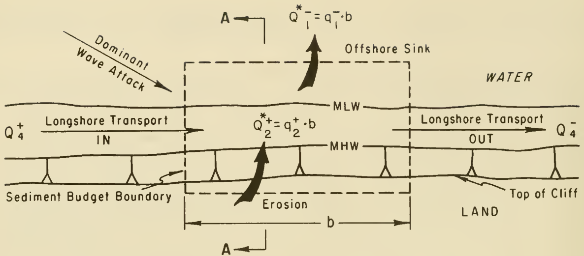
ERODING SHORELINE - PLAN VIEW (Not to Scale)
