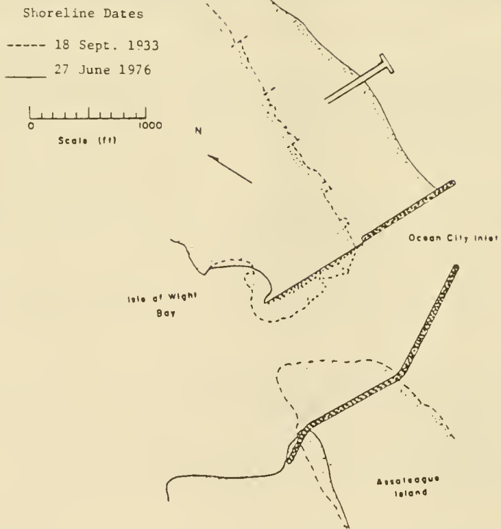
Figure 1-9. Littoral barrier, Ocean City Inlet, Maryland (after Dean and Perlin, 1977).
