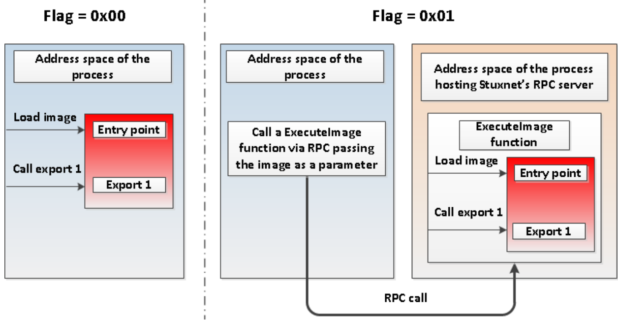
Figure 4.4.4 – Dispatching Received Data
