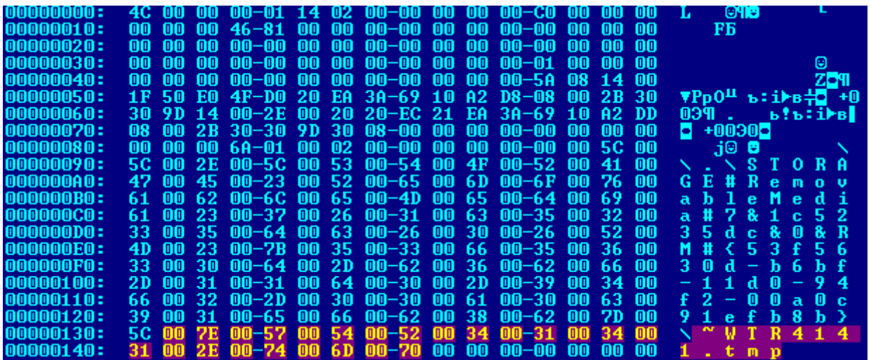
Figure 3.2.2 – Contents of the .LNK Files
