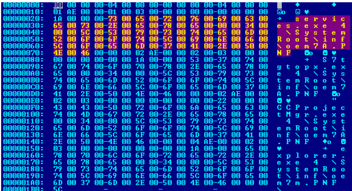
Figure 4.2.3 – The configuration data of the driver
