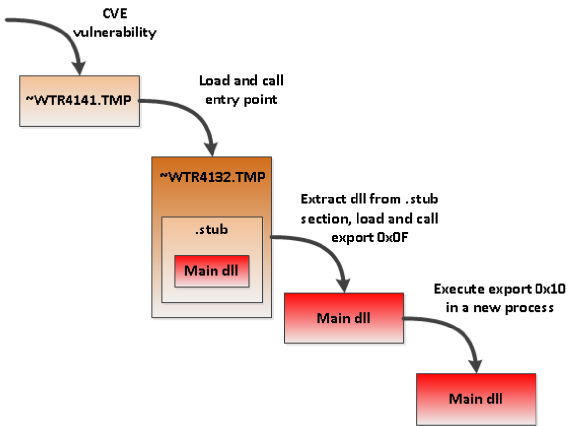
Figure 4.1.7 – Installation of the Malware
