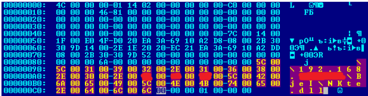
Figure 3.1.8 – .LNK File Generated by Metasploit
